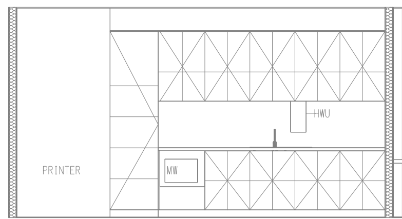
DETAIL A KITCHENETTE ELEVATION SCALE 1:50
