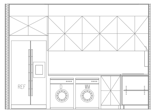
DETAIL C UTILITIES BENCH ELEVATION 2 SCALE 1:50
